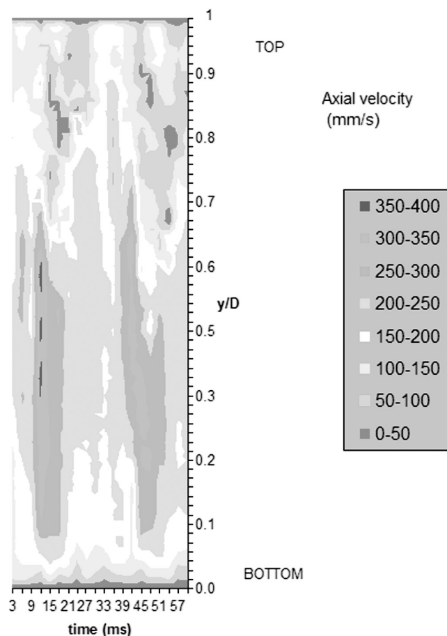
Figure 4. Space–time diagram of the axial velocity component for an impeller speed of 1200 rpm and \phi = 5\% .
