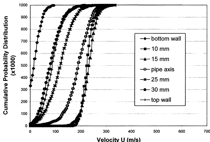
Figure 7. Cumulative probability distribution function (CPDF \times 1000 ) on velocities for an impeller speed of 1200 rpm and \phi = 20\% .
