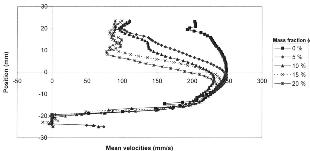
Figure 5. Mean axial velocity profiles for different mass fractions \phi of the dispersed phase and for an impeller speed of 1200 rpm.
